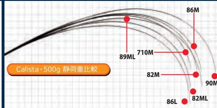
Calista / Bending Curve / Load 500g
