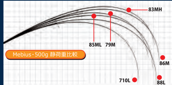
Various / Bending Curve / Load 500g
